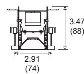
9/16" Screw Slot Ceiling
