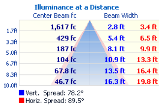
SS-8-L108-SC
