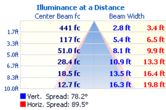
SS-2-L27-SC
