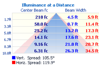
SS-3-L13-RC
