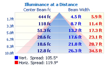
SS-2-L27-RF
