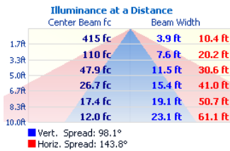
SS-2-L36-SF
