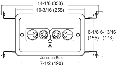
All dimensions are in inches (millimeters).
