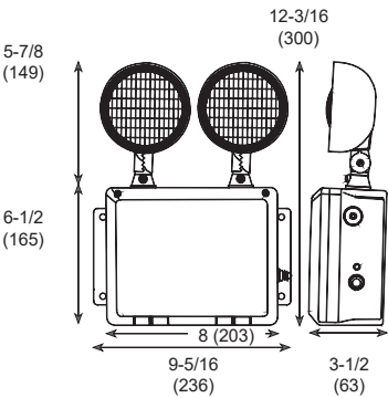
All dimensions are in inches (millimeters).
