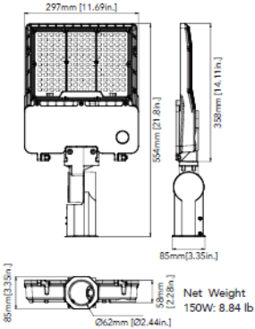
150W (Slip Fitter Mount)
