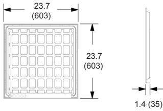
Specifications: ULP-2G 2'x2'
