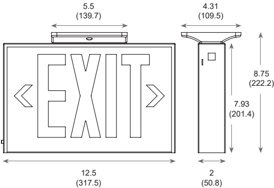
All dimensions are in inches (millimeters).
