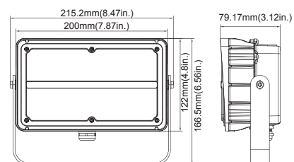
60W(Trunnion Mount)
