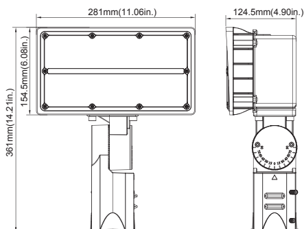
100W(Slipfitter Mount)
