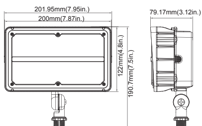
60W(Knuckle Mount)
