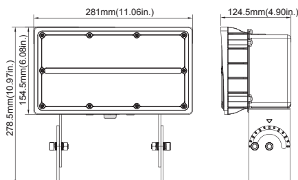
100W(Yoke Mount)
