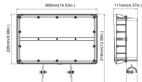
200W(Yoke Mount)
