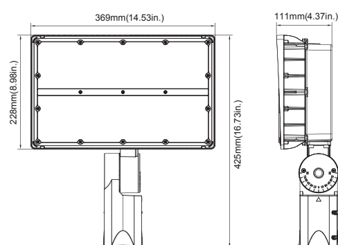
200W(Slipfitter Mount)
