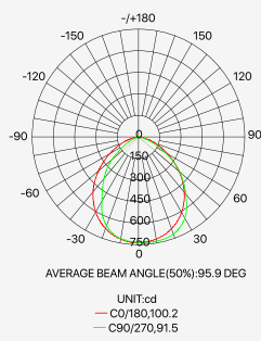
LUMINOUS INTENSITY DISTRIBUTION DIAGRAM
