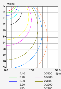
C0 PLANE ISOLUX DIAGRAM (UNIT:lx)
