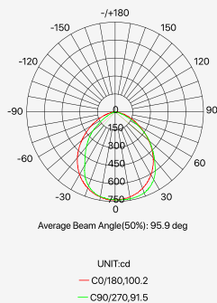
LUMINOUS INTENSITY DISTRIBUTION DIAGRAM
