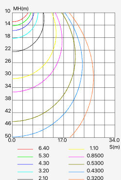
C0 PLANE ISOLUX DIAGRAM (UNIT:lx)
