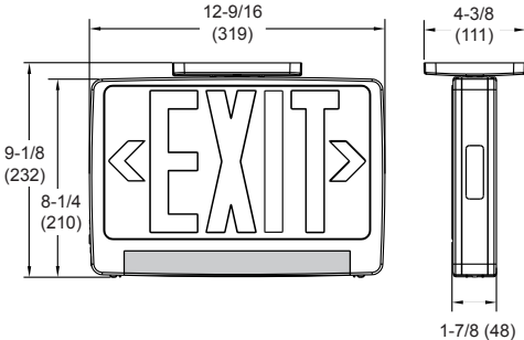
All dimensions are in inches (millimeters).
