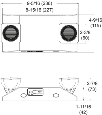
All dimensions are in inches (millimeters).
