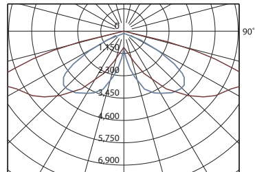
Polar Candela Distribution (TYPE 3 medium + House Shield)
