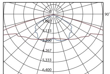
Polar Candela Distribution (TYPE 3 medium)
