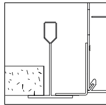
15/16" Grid Mounting Options
