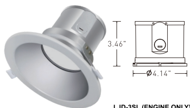
LJD-3SL (ENGINE ONLY)
