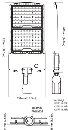
(Slip Fitter)
