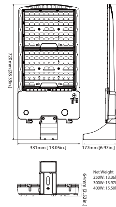
(Pole Mount)
