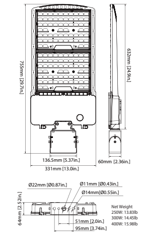
(Trunnion Mount)
