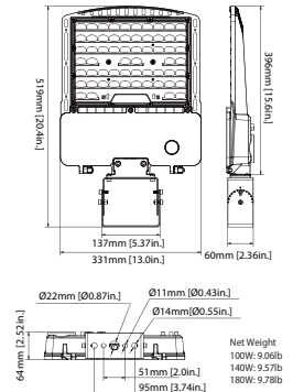
(Trunnion Mount)
