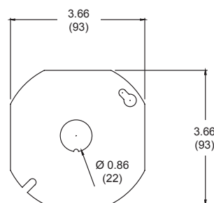
JC4 : Octagon cover plate
