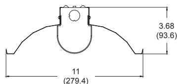
SYM : Symmetric Reflector
