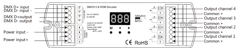
4DMX (4-channel DMX decoder)
