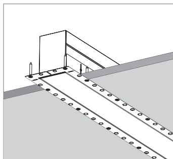
Recessed Mud-In Drywall Ceiling (Trimless)
