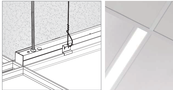
Mount by T-grid hooks to secure in T-grid ceiling / Drop ceiling
