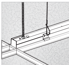
G1 Mounting option
