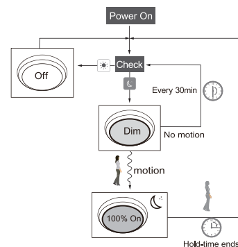
The light remains in dimming level at night.
