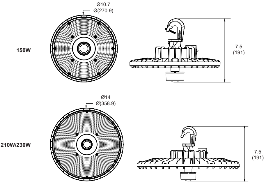
All dimensions are in inches (millimeters).
