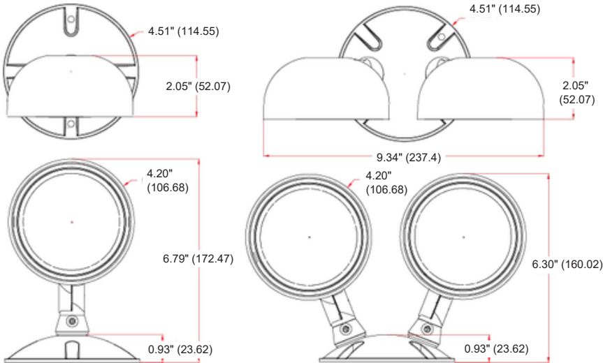
All dimensions are in inches (millimeters).
