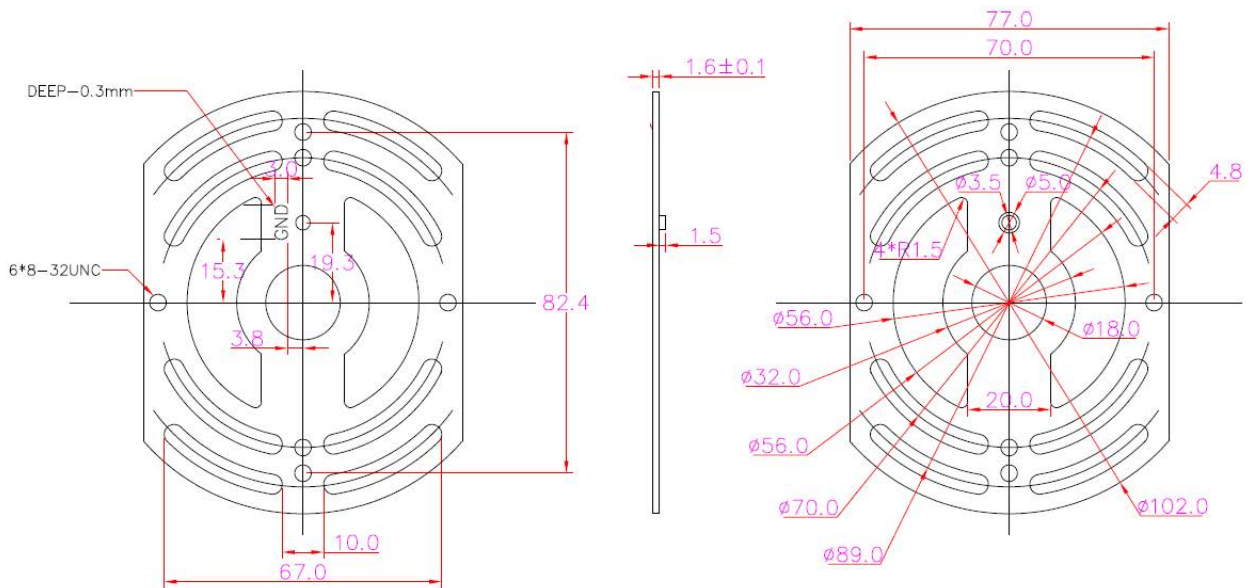
Dimensions for FIGURE D shown in mm.
