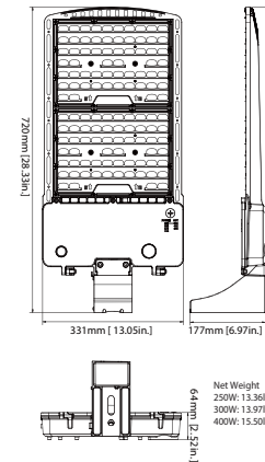
(Pole Mount)
