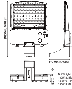
(Pole Mount)
