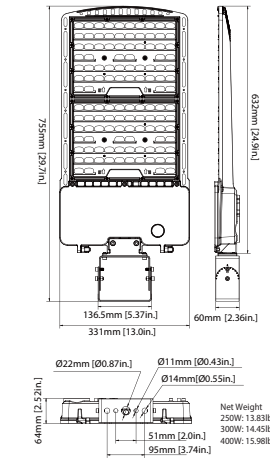
(Trunnion Mount)
