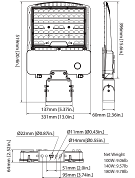
(Trunnion Mount)
