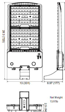
(Pole Mount)
