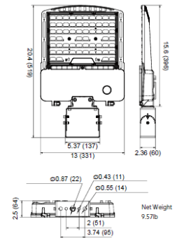
(Trunnion Mount)
