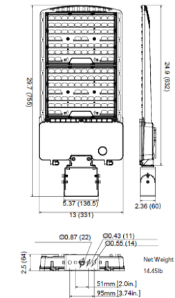
(Trunnion Mount)
