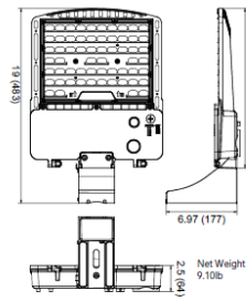
(Pole Mount)
