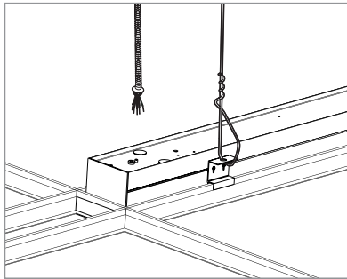
T-Grid Hook
