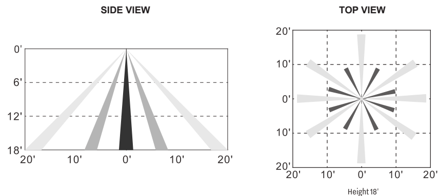
ADPMS, IFS105SE coverage pattern
