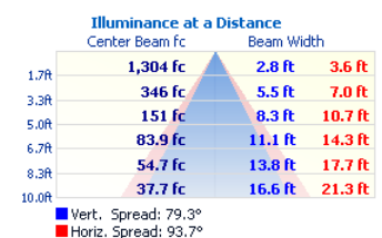
CUBE4-8-D48L-WW
