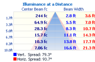
CUBE4-2-D36L-WW
