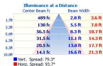
CUBE4-4-D36L-WW
