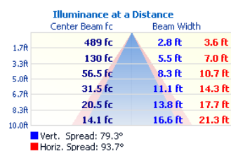
CUBE4-8-D18L-WW
