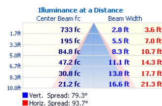
CUBE4-8-D27L-WW
