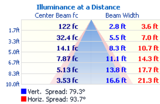
CUBE4-2-D18L-WW
