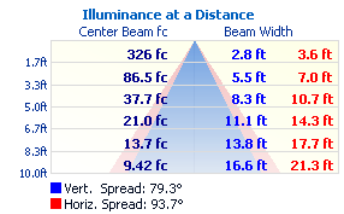
CUBE4-2-D48L-WW
