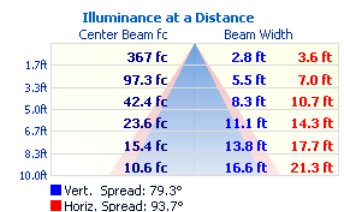
CUBE4-6-D18L-WW
