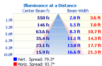
CUBE4-6-D27L-WW
