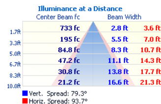
CUBE4-6-D36L-WW
