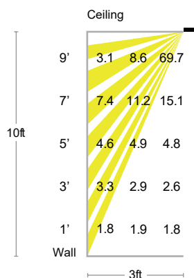
CUBE4-4-D18L-WW
