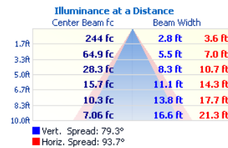
CUBE4-4-D18L-WW
