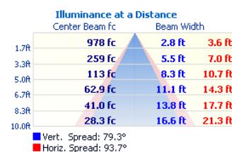
CUBE4-8-D36L-WW
