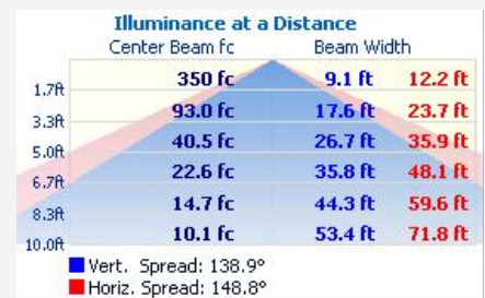
LPT-9-2G3SH (120W)
