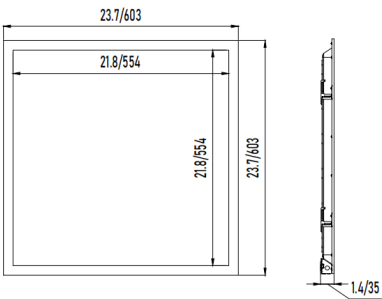
Specifications: 2'x2'
