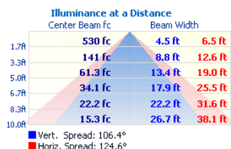
DW-LP-4-36LED
