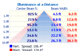
DW-LP-4-56LED
