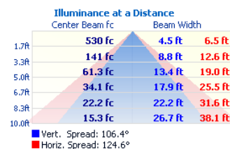
DW-LP-2-36LED
