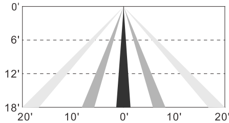
ADPMS, IFS105SE coverage pattern
