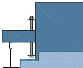
Swing gate hanger range 0.9in(25mm) - 3.1in (80)mm
