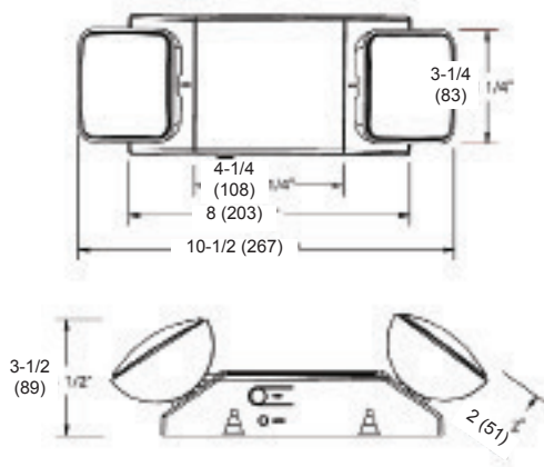
All dimensions are in inches (millimeters).
