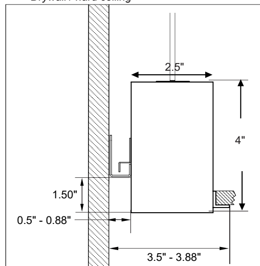
Flushed Lens w/ NF* mounting type (1/2" flange on one side) Drywall / hard ceiling
