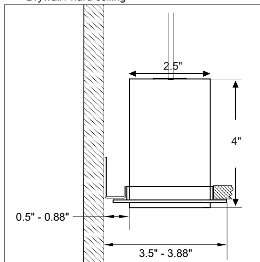
Flushed Lens w/ Fixed* mounting type (1/2" flange on both sides) Drywall / hard ceiling
